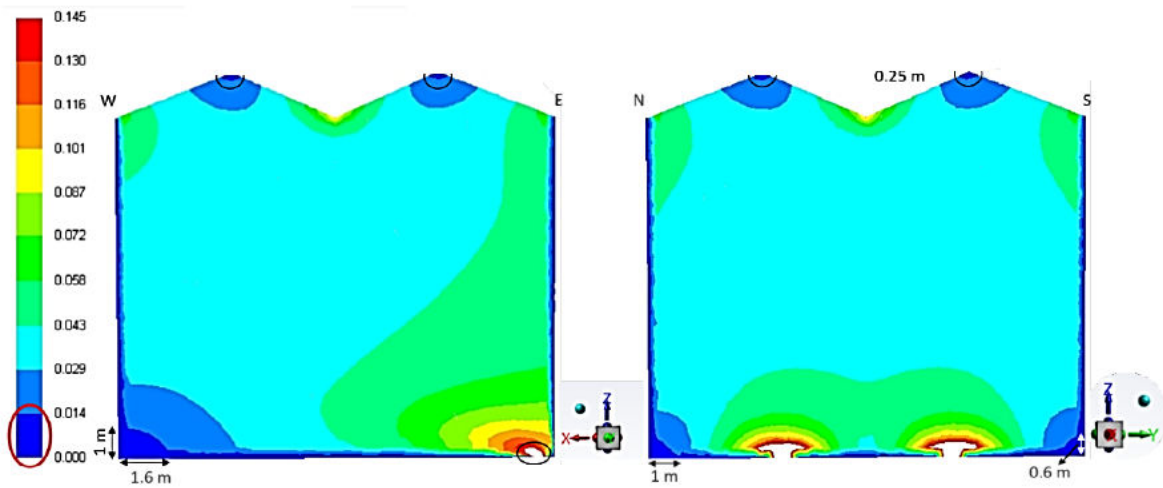
Figure 29. Airflow through grain with 16 t removed and 5 kW fan.
