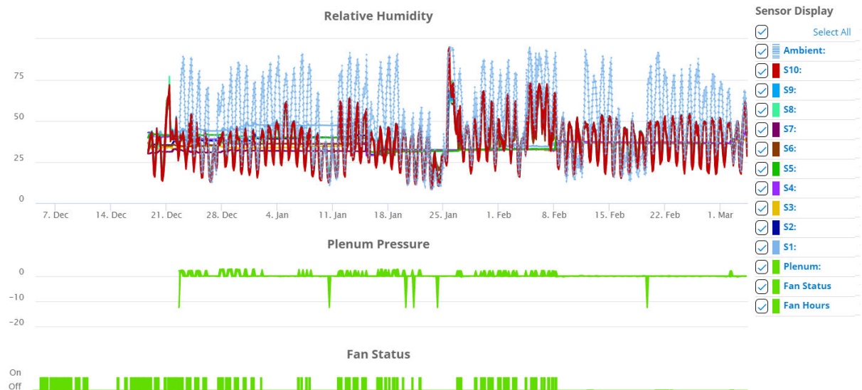
Figure 9. Long term humidity trends in white painted silo: In grain = S1 to S6; headspace = S7 to S10.
