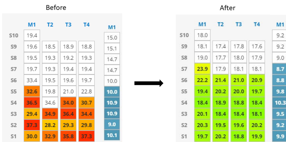
Figure 16c : Aeration cooling of 1,000 t white pained silo with 5 kW fan Barley = 140 fan hours from 5/12/20 to 12/12/20
