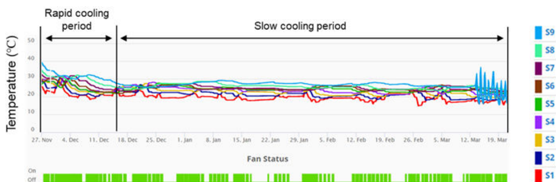
Figure 17. Example of multiple reheatings of grain (sensor S1 at bottom) during storage.
